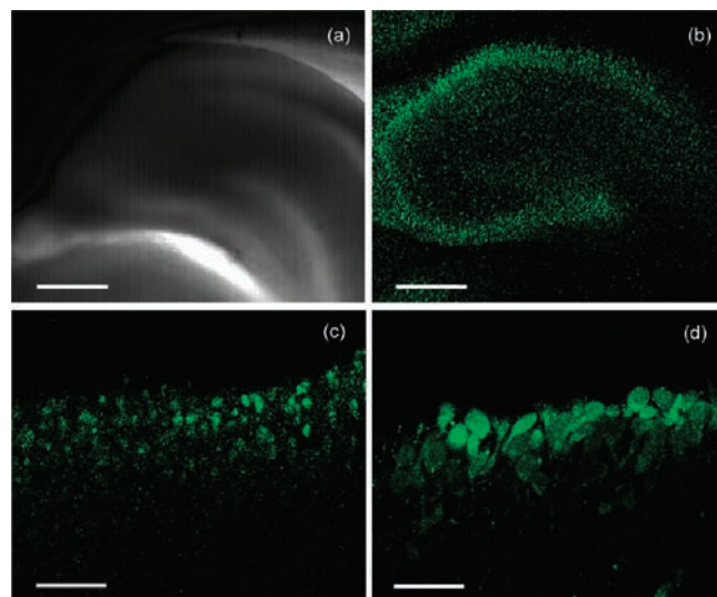
FIGURE 3. Images of a fresh mouse hippocampal slice stained with 5 \mu M AMg1-AM: (a) bright-field image shows the CA1 and CA3 regions as well as the dentate gyrus by magnification at 10 \times ; (b) TPM image with the same magnification reveals the same regions at a depth of \sim 270 \mu m; (c) magnification at 40 \times shows the CA1 layer at a depth of \sim 150 \mu m; (d) magnification at 100 \times shows CA1 pyramidal neurons at a depth of \sim 150 \mu m. Scale bars = 300 (a, b), 120 (c), and 30 (d) \mu m. The TPEF images were collected at 500–620 nm upon excitation at 780 nm with femtosecond pulses.
