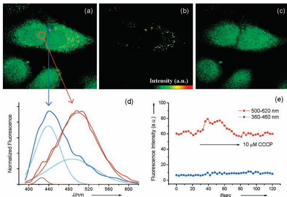
FIGURE 2. TPM images collected at 360–620 (a), 360–460 (b), and 500–620 nm (c) of AMg1-AM-labeled (2 \mu M) Hep3B cells. (d) Two-photon excited fluorescence spectra from the hydrophobic (blue) and hydrophilic (red) domains of AMg1-AM-labeled Hep3B cells. The excitation wavelength is 780 nm. Cells shown are representative images from replicate experiments. (e) TPEF intensity collected at 500–620 nm (red) and 360–460 nm (blue) before and after addition of CCCP as a function of time.
