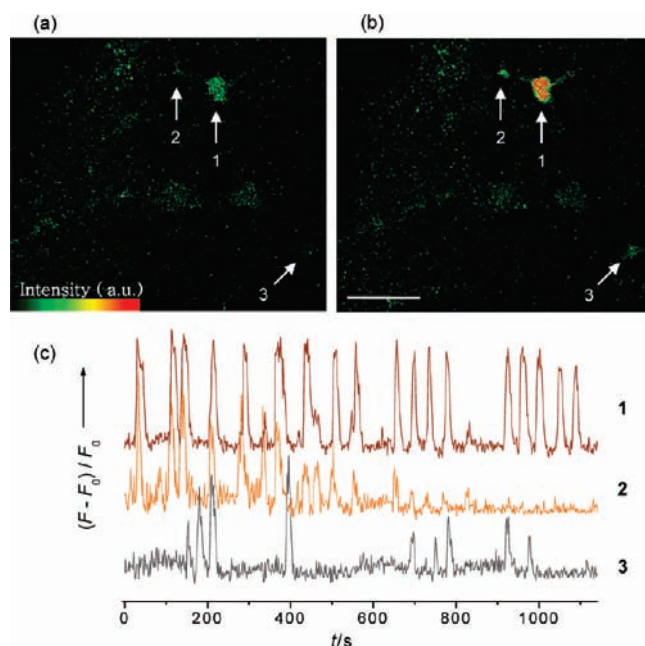
FIGURE 4. Pseudocolored TPM images of a fresh rat hypothalamic slice stained with 10 \mu\text{M} ACa1-AM taken after 195 (a) and 214 (b) s. Magnification at 100 \times shows hypothalamic area at a depth of \sim 170 \mu\text{m} . (c) Spontaneous \text{Ca}^{2+} transients recorded in soma (1), astrocyte process (2), and neighboring cell (3). The TPEF images were collected at 500–620 nm upon excitation at 780 nm with femtosecond pulses. Scale bar, 30 \mu\text{m} .
